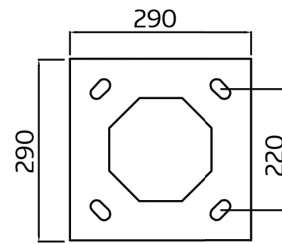
BASE PLATE
