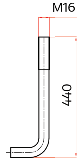
M16 x 500 Anchor Bolts ... 4 pcs
